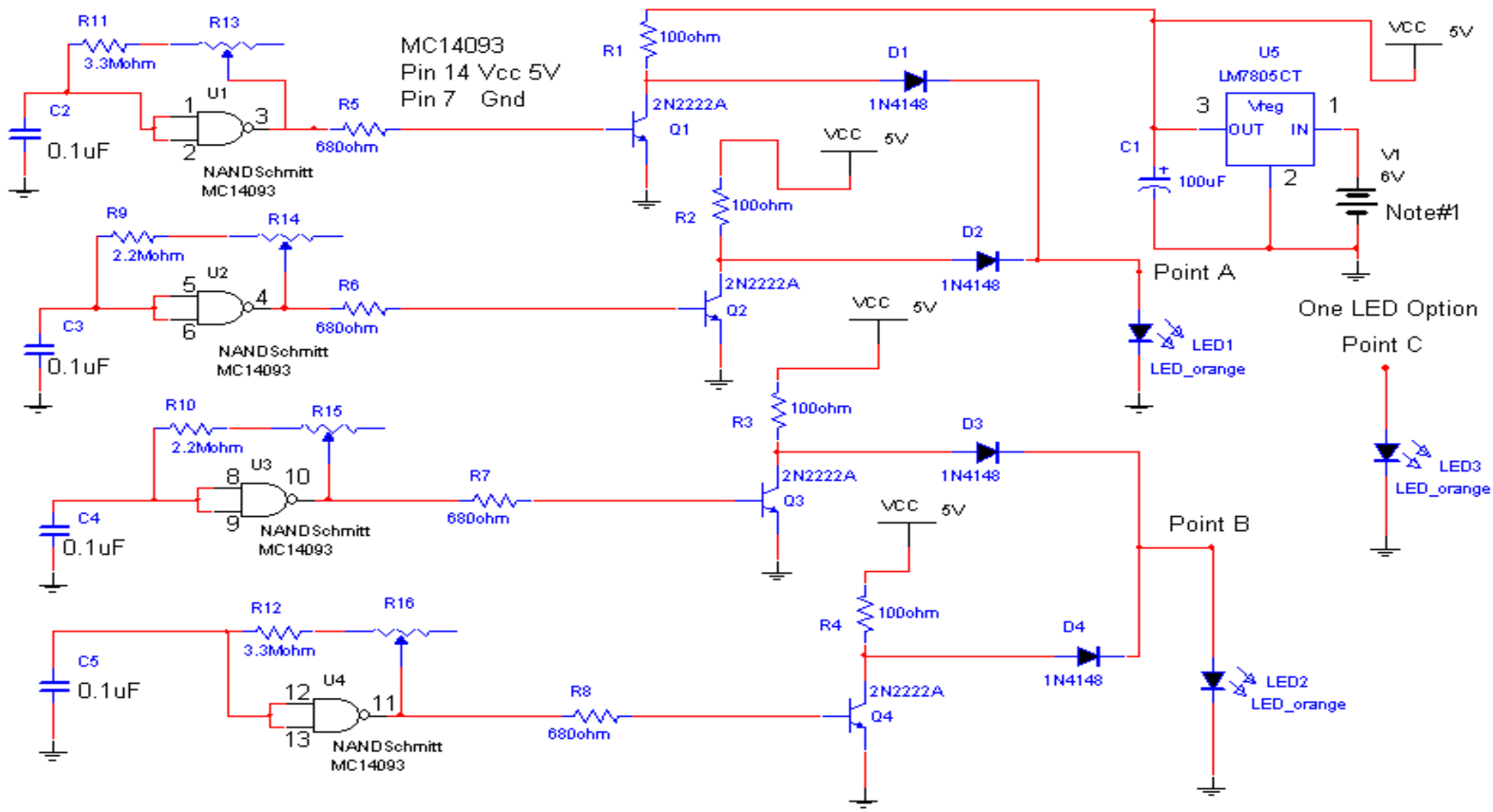
Pumpkin Light LED Large Schematic
